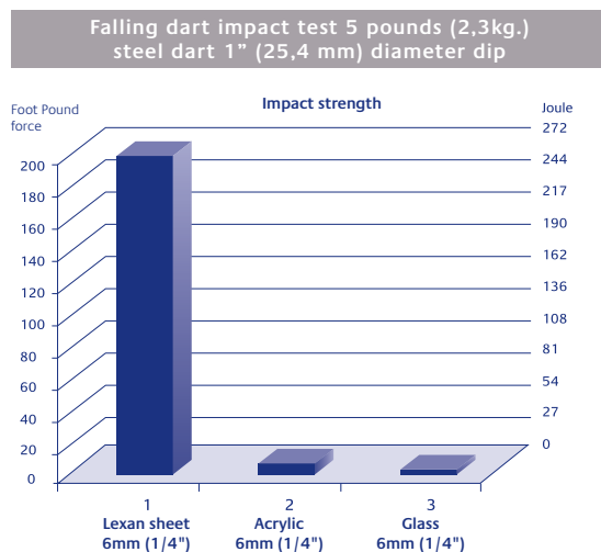
Figure 1 Impact resistance
